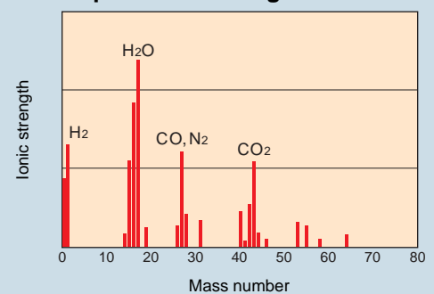
Mass spectrum of out gas
