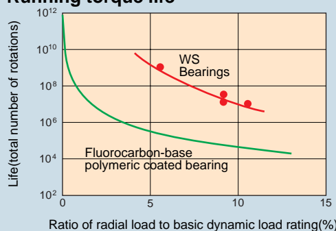
Running torque life
